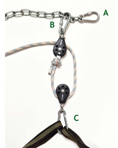
Figure 6 The different carbine hooks and their placements.
